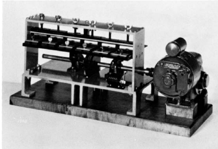
FIG. 1 Ross Flexing Machine
